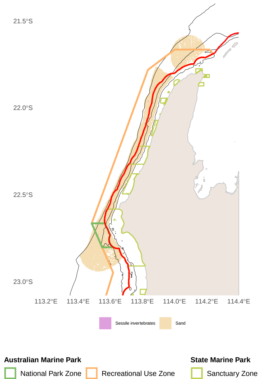
Figure 2: Predicted dominant habitat type from stereo-BRUV groundtruthing. Commonwealth marine park boundaries are shown. The red line delimits state and commonwealth waters. Bathymetric contour at 30 m is shown.
